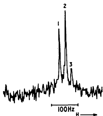
Fig. 3. 36.4 MHz ^{31}\text{P} -NMR spectrum at 18 °C of sonicated vesicles prepared from the total polar lipids isolated from membranes of 0.12 mM oleic acid-grown A. laidlawii cells. Chemical shifts down field of the ^{31}\text{P} resonance of triphenyl phosphine in chloroform are 6.5, 5.8 and 5.3 ppm for resonances 1, 2 and 3, respectively.
